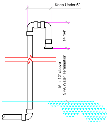
Air Venturi Detail
